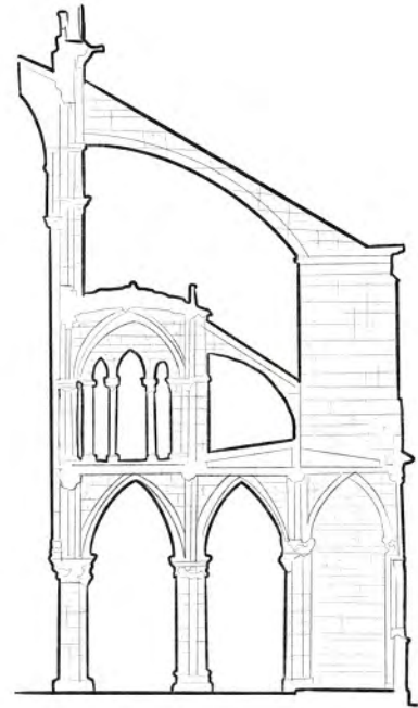
↑ Arc-boutant
